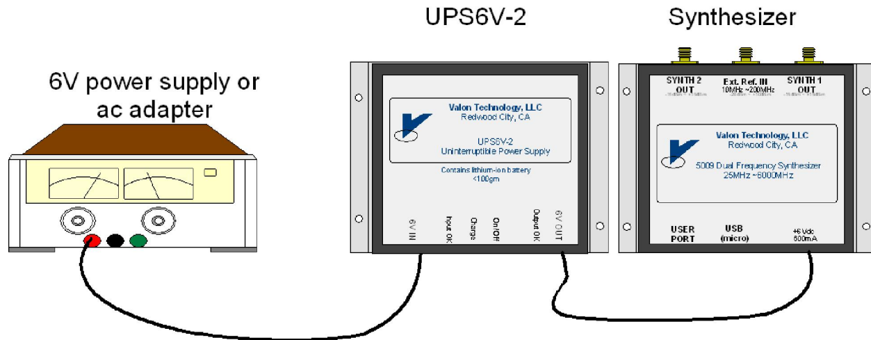
Figure 2 Typical Setup
